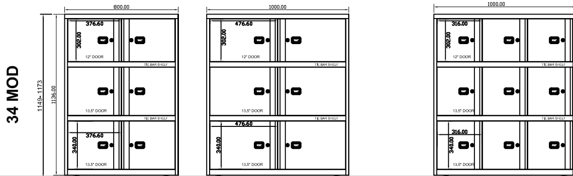
SYL0834LSA2B HEIGHT 34 MOD x 800w c/w 2 x 12" + 4 x 13.5" DOORS
