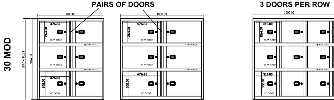
SYL0830LS2JA HEIGHT 30 MOD x 800w c/w 4 x 10.5" + 2 x 12" DOORS
