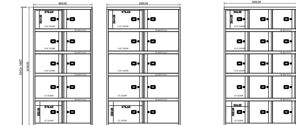
SYL0850LS3J2A HEIGHT 50 MOD x 800w c/w 6 x 10.5" + 4 x 12" DOORS
