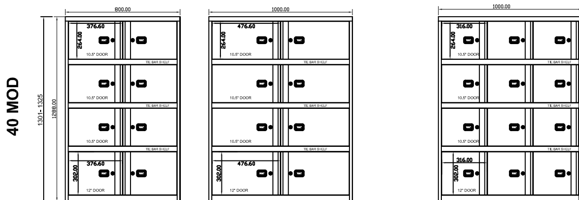
SYL0840LS3JA HEIGHT 40 MOD x 800w c/w 6 x 10.5" + 2 x 12" DOORS
