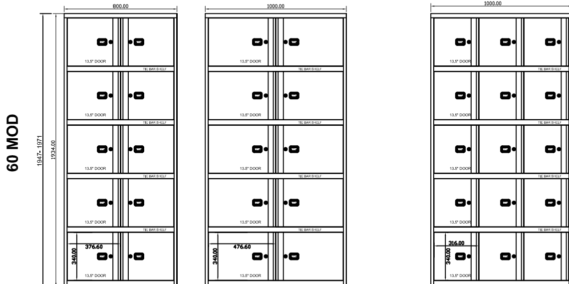
SYL0860LS5B HEIGHT 60 MOD x 800w c/w 10 x 13.5" DOORS
